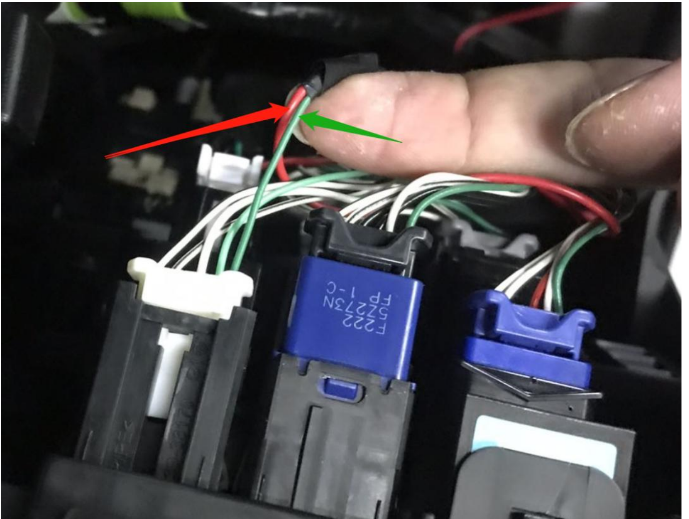
15.前开关ILL红色小灯线接箭头绿色线Front switch ILL red light cable connected to arrow green cable
