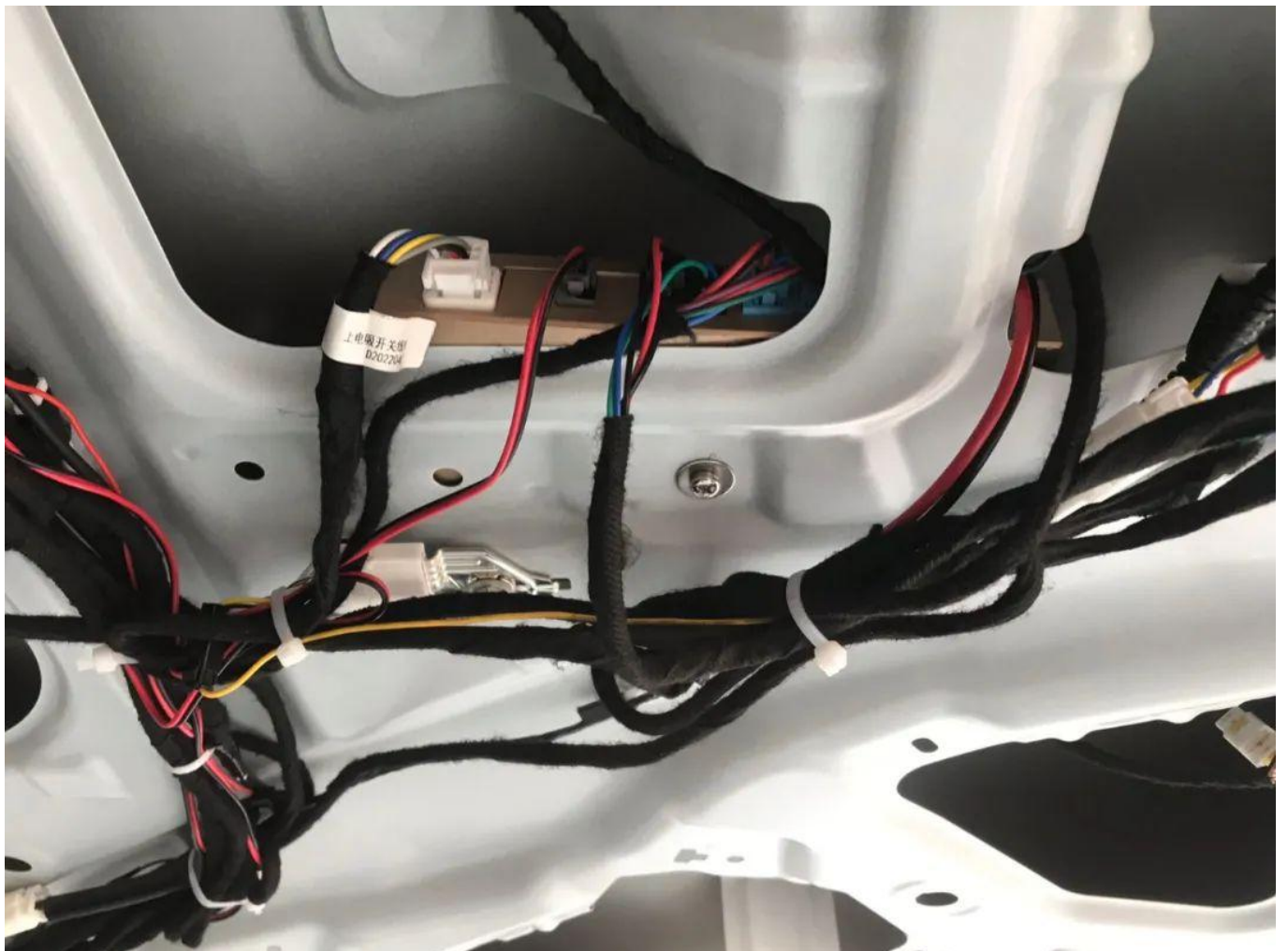
9. 如下图ECU控制盒用螺丝固定在尾门内侧 As shown below, the ECU control box is fixed with screws on the inside of the tail door
