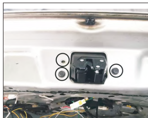
6. Abort the original screw, remove the original car door lock, installed on our electric absorption, use the original car screws
