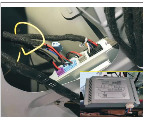
8. The hole line, power line, electric line plug according to the color of a pair of control box
