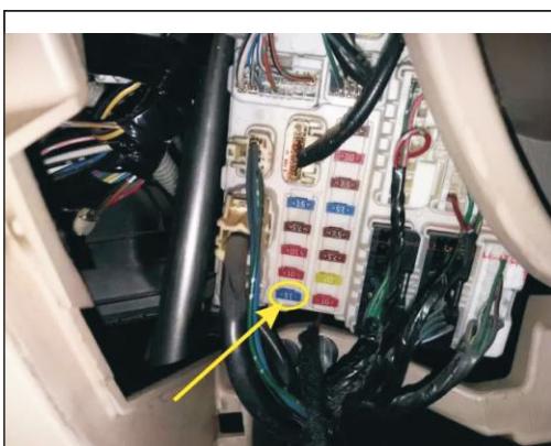
4. On the right side of the main driving 15 a fuse, unplug the original car plug in our power plug
