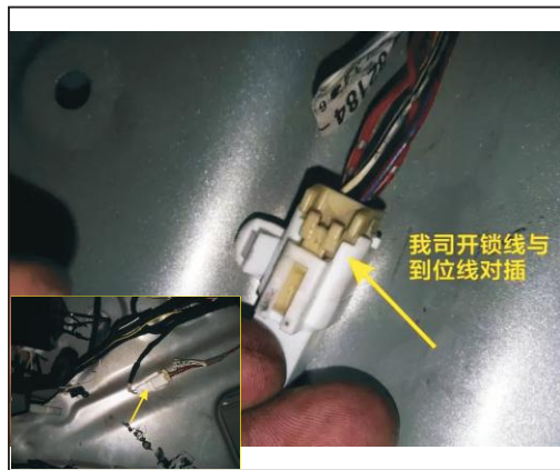
10. In the tail gate to find the original socket, we lock line socket
